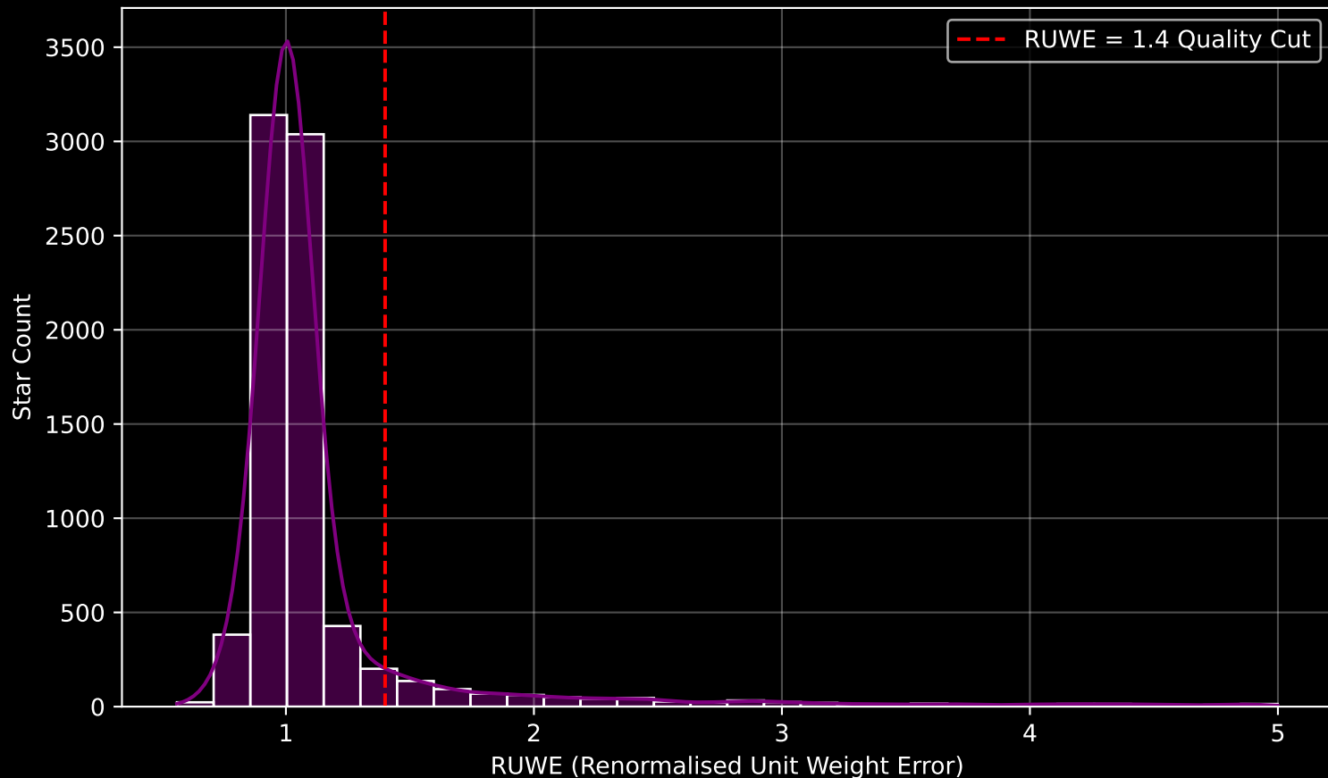
GALAH DR4 Field [-5] RUWE Distribution (n= 7977)
