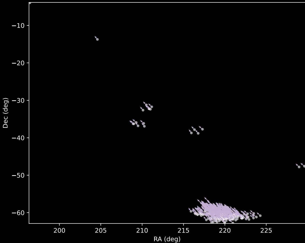
GALAH DR4 Cluster 209 Proper Motion Vectors (n=255)
