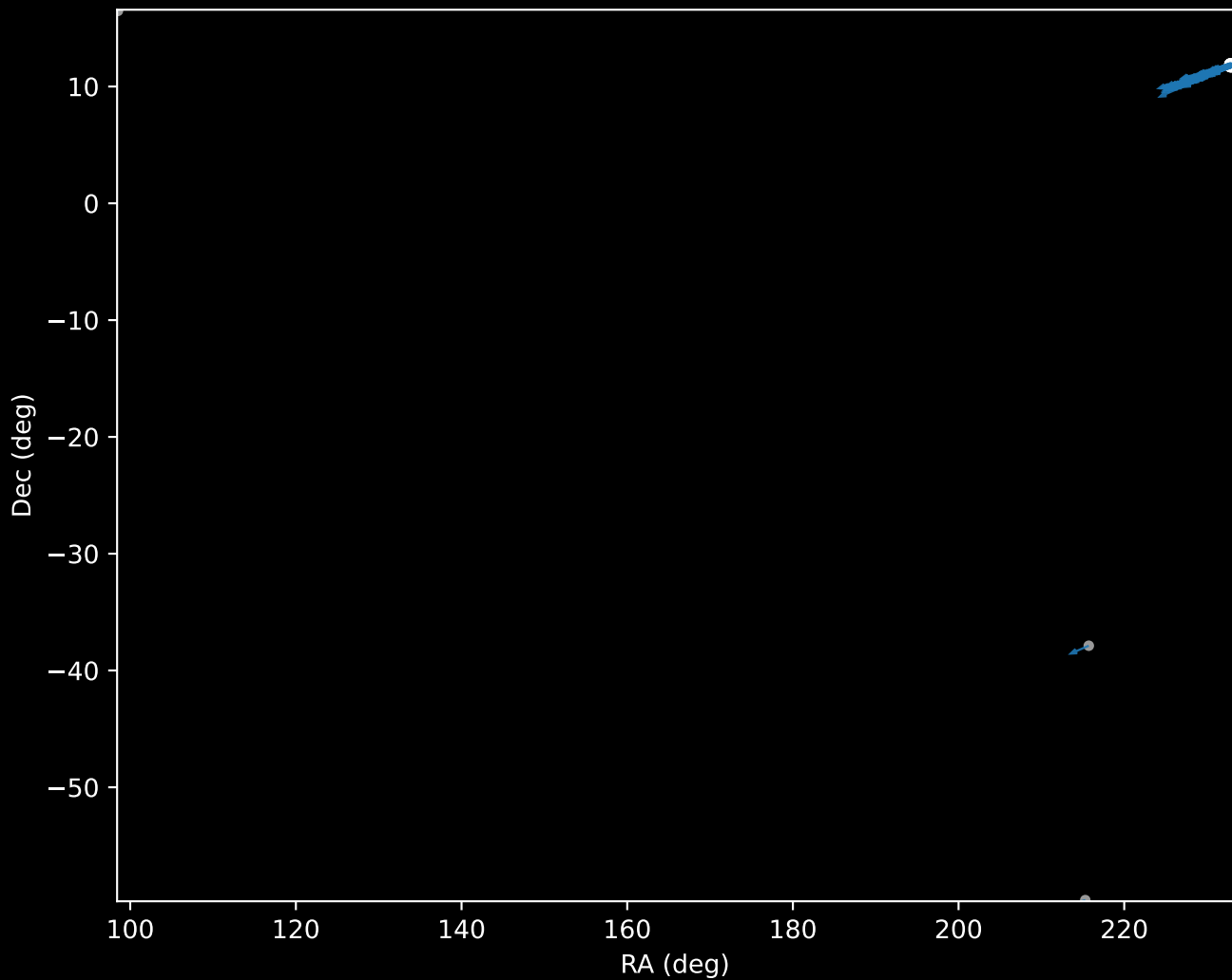
GALAH DR4 Cluster 160 Proper Motion Vectors (n=179)
