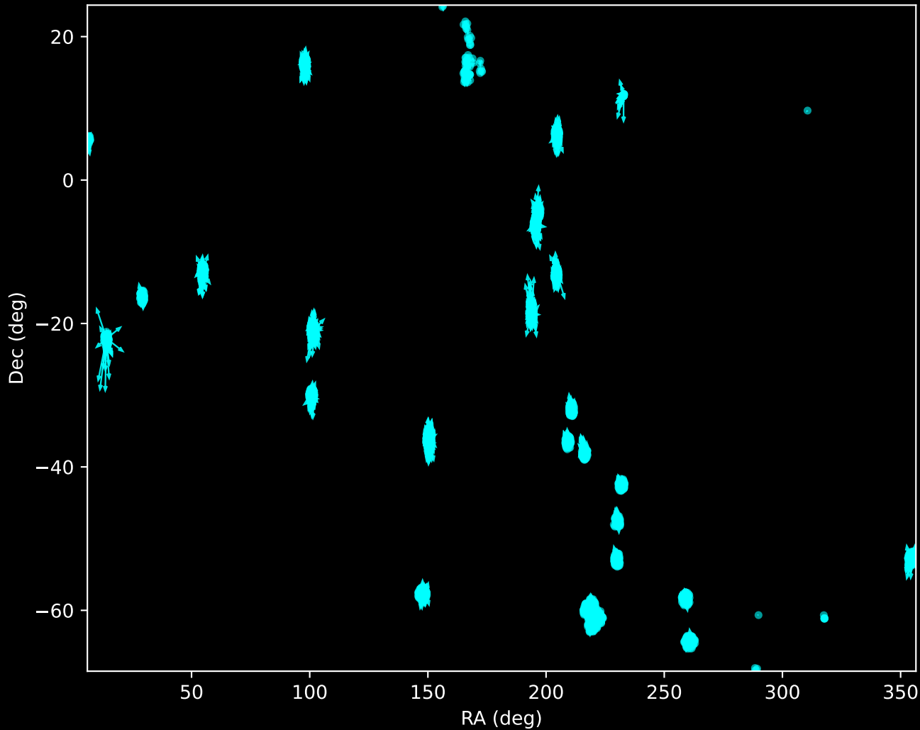
GALAH DR4 Noise Stream Proper Motion Vectors (n=2750)
