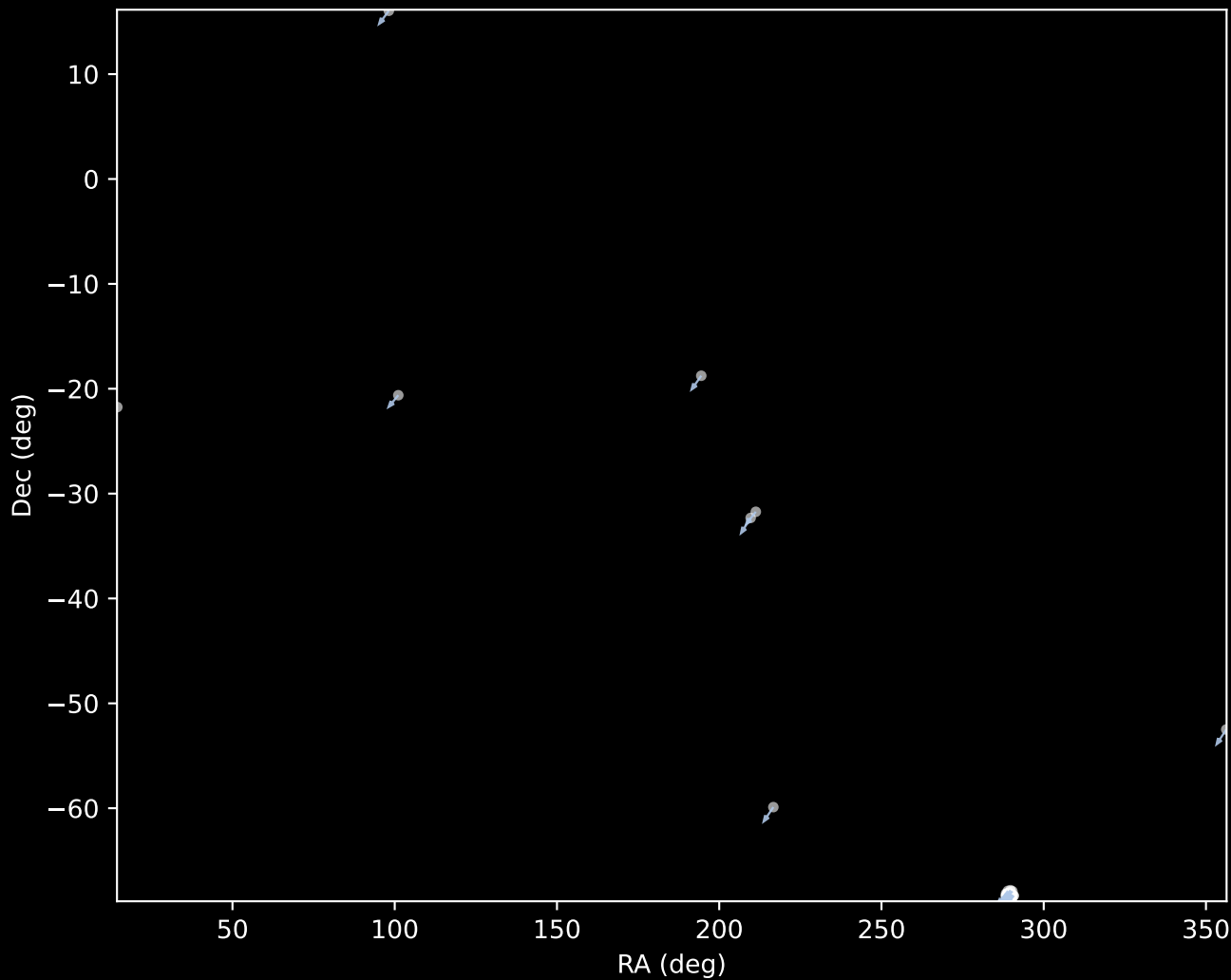
GALAH DR4 Cluster 241 Proper Motion Vectors (n=224)
