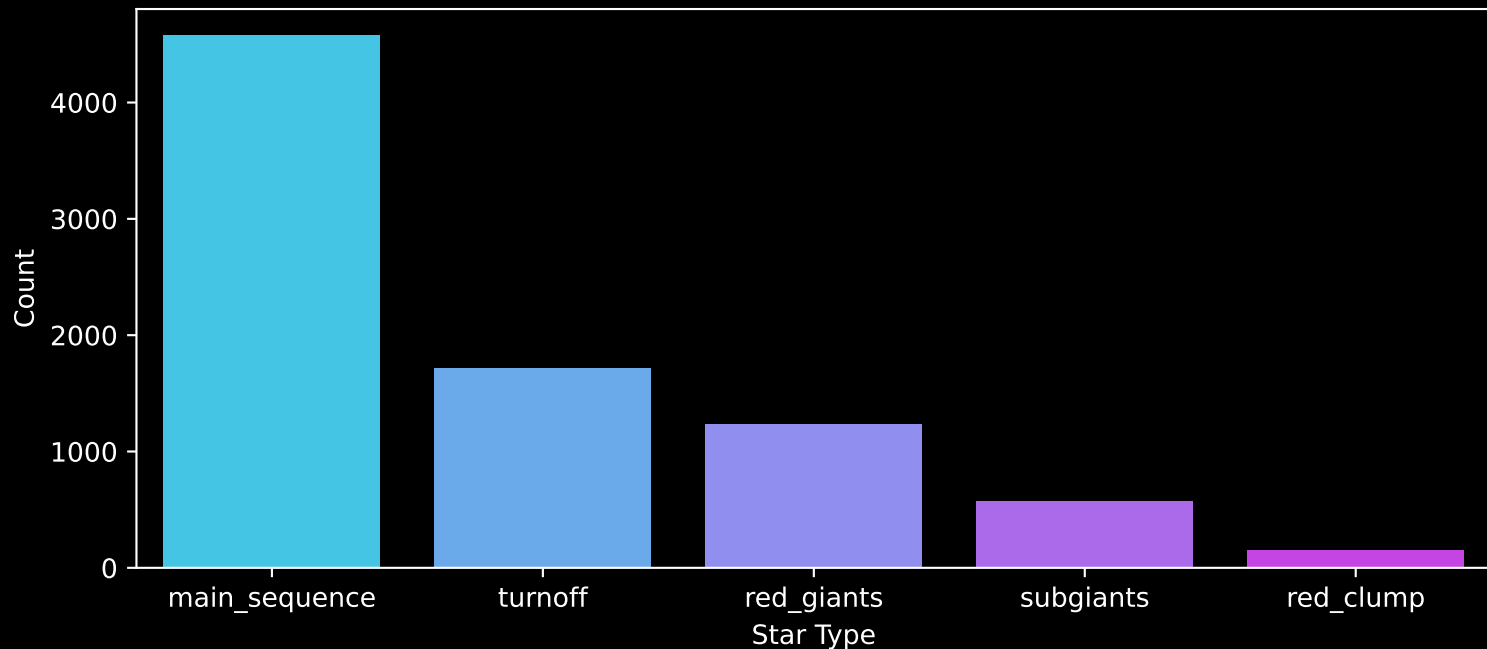
GALAH DR4 Field: [-5] Count plot of Star Type
