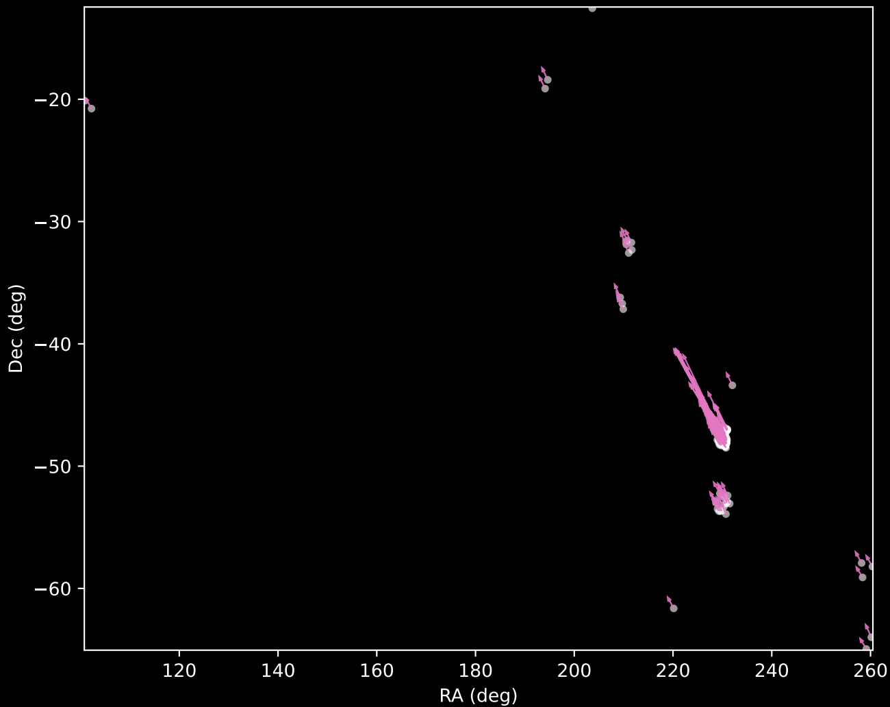
GALAH DR4 Cluster 332 Proper Motion Vectors (n=154)
